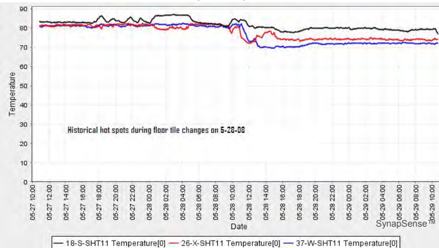
rack-top temperatures
