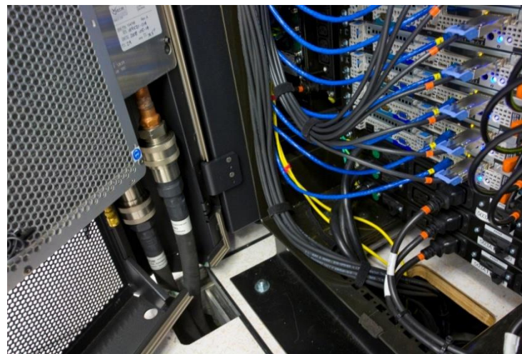
液体冷却连接管道Liquid Cooling Connections
