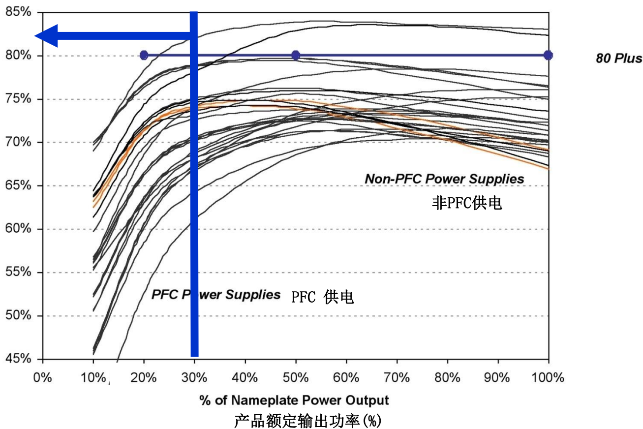
测量到的服务器电源供应效率 (所有的因素) Measured Server Power Supply Efficiencies (all form factors)
