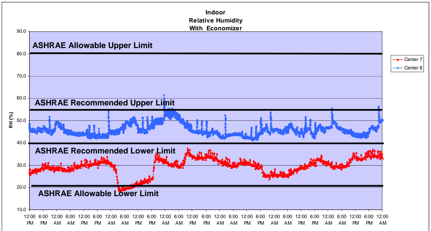
Figure 27: Humidity at server rack for data centers with economizers
