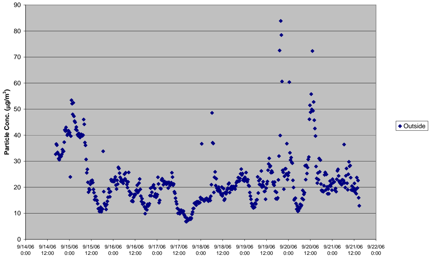
Figure 6: Center 3 outdoor particle concentration
