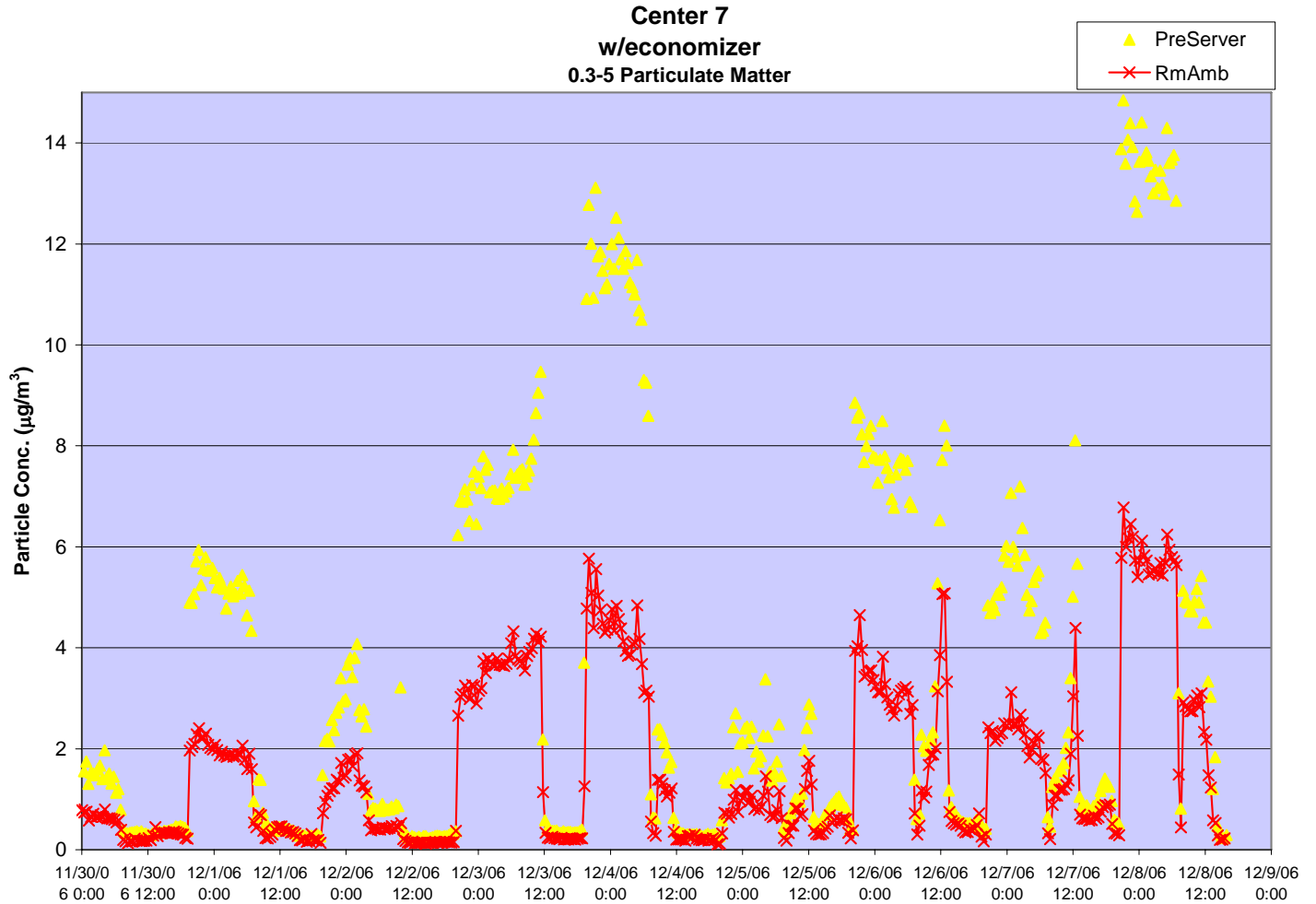
Figure 22: Center 7 outdoor particle concentration with economizer
