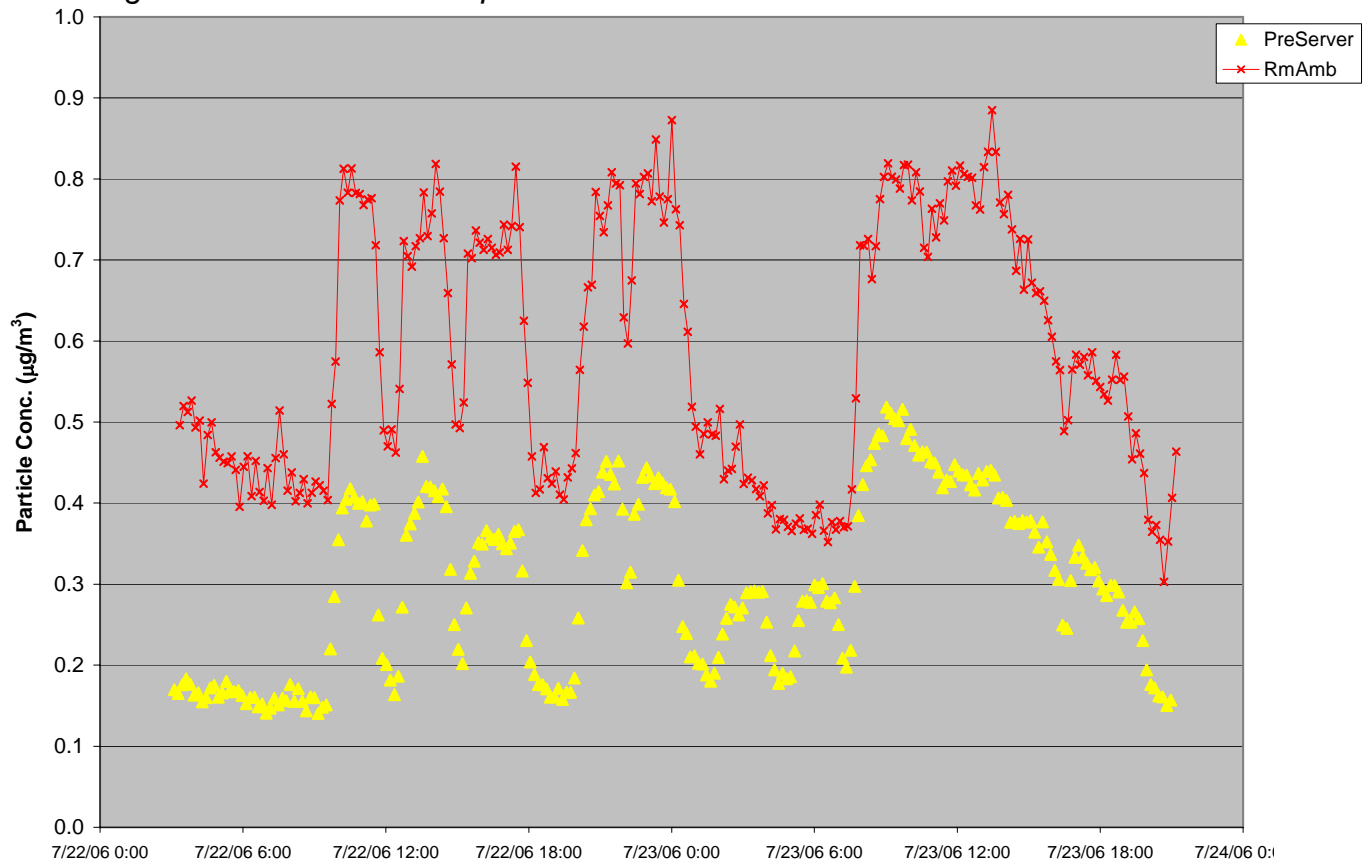
Figure 16: Center 7 indoor particle concentration
