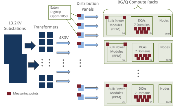
Figure 2: Power measurement locations for the Mira supercomputer
