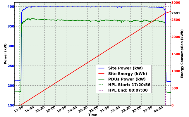
Figure 5: Power and energy measurements during the Colosse run
