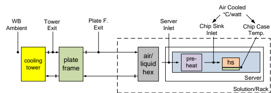
Figure 5: Cooling Tower with Air Cooling at the Chip
