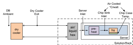
Figure 6: Dry Cooler with Air Cooling at the Chip
